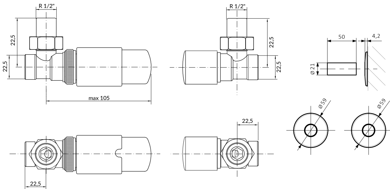
Thermostatventil
