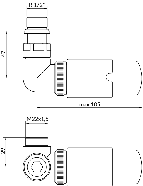
Winkeleck-Thermostatventil
